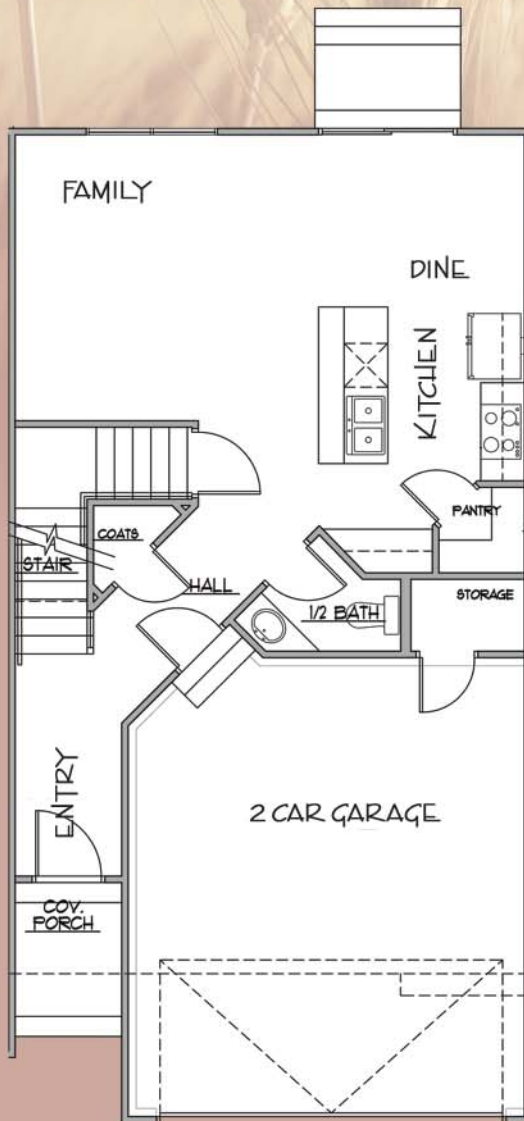
MAIN FLOOR
